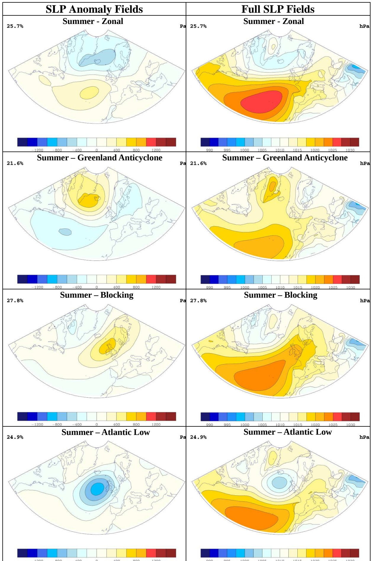
Data : Daily Era-Interim Sea Level Pressure – JJA 1981-2010
